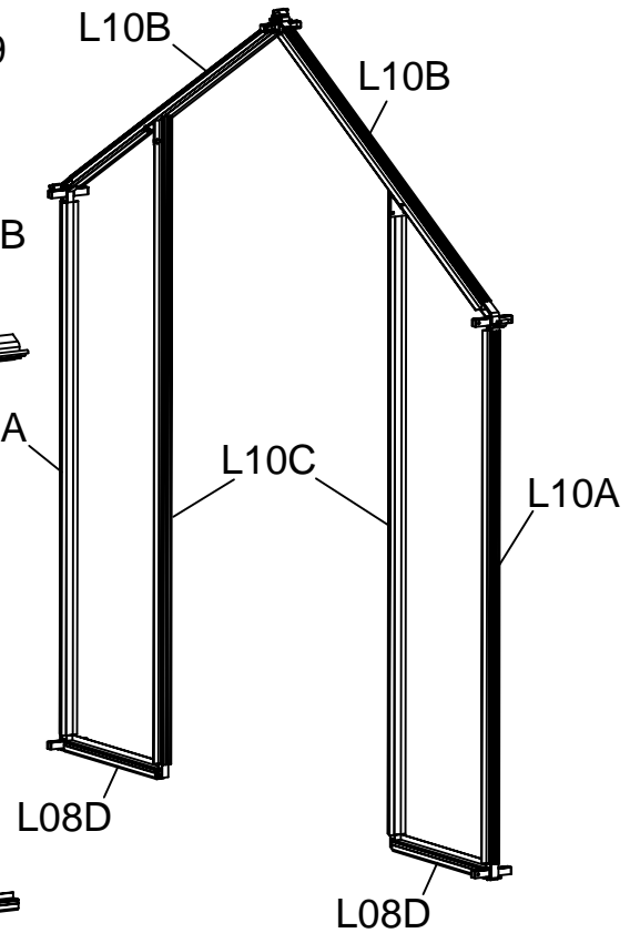
Middle Section Assembly Instruction
