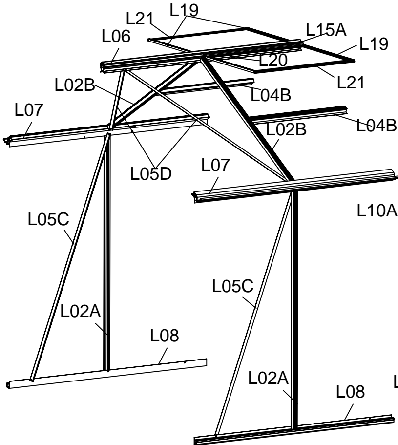
2 Sections Assembly Instruction
